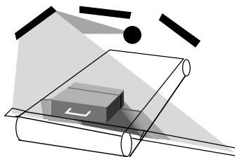
Figure 3.32. Concept giving views with horizontal rotation in stead of horizontal shear. The x-ray source exposes the x-ray mirrors one after another. In total 16 such mirrors are required to get 16 views. Only 3 are shown.
