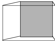
Figure 3.12a. With HC VP perspective the height of the front and back plane are equal, while the width of the front plane is greater than that of the back.
