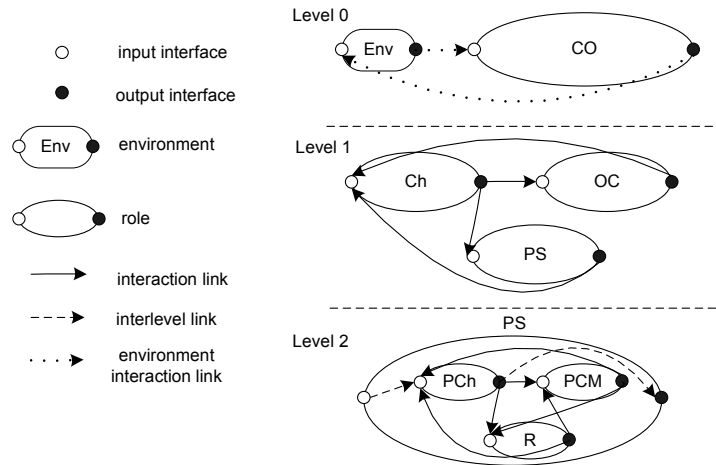
Figure 1. Model of the conference organizing committee
