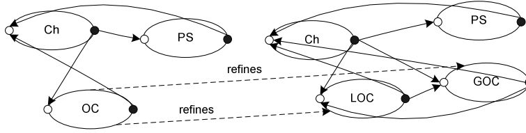
Figure 2. Example of Role refinement operator application
