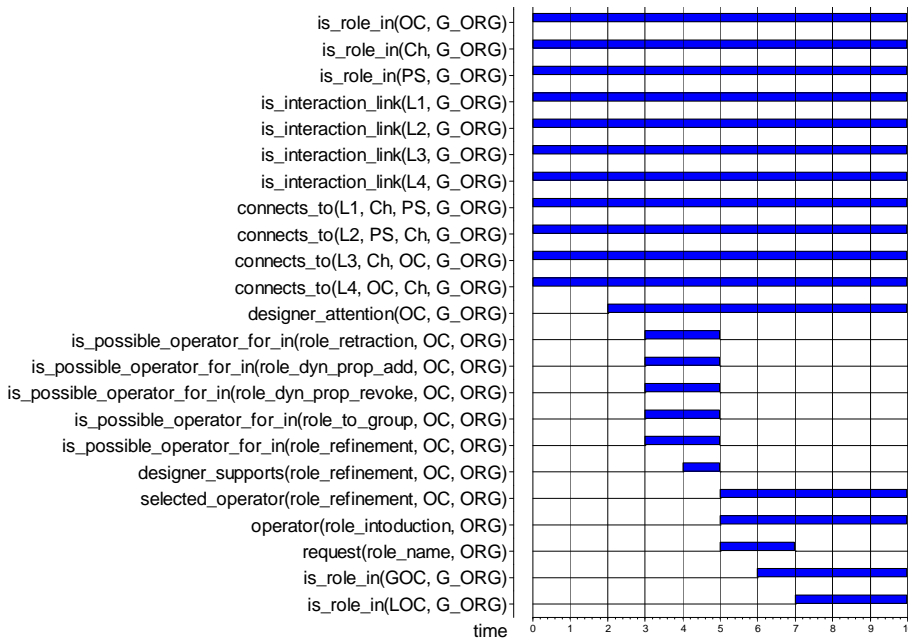
Figure 4. Screen print of a trace illustrating dynamics of the design process for role refinement
