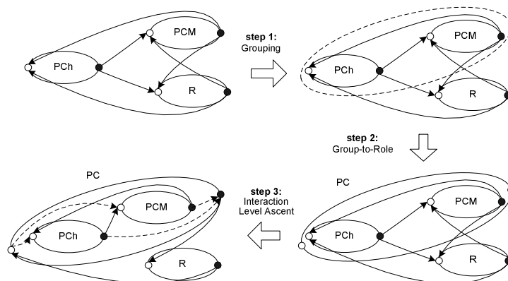
Figure 3. Example of Role refinement operator application
