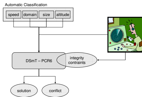
Figure 4 Basic system architecture to combine classification solutions
