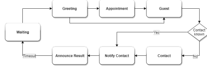
Fig. 2: Reception Dialogue States
