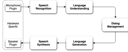
Fig. 1: Agent Architecture
