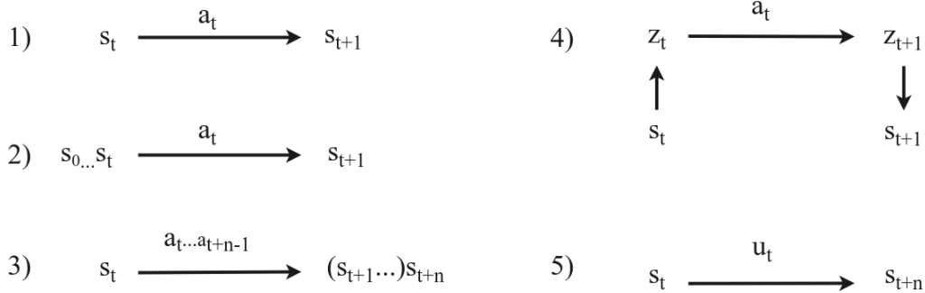
Figure 2: Overview of different types of mappings in model learning. 1) Standard Markovian transition model s_t, a_t \rightarrow s_{t+1} . 2) Partial observability (Section 4.4). We model s_{0...s_t}, a_t \rightarrow s_{t+1} , leveraging the state history to make an accurate prediction. 3) Multi-step prediction (Section 4.6), where we model s_t, a_t...a_{t+n-1} \rightarrow s_{t+n} , to predict the n step effect of a sequence of actions. 4) State abstraction (Section 4.7), where we compress the state into a compact representation z_t and model the transition in this latent space. 5) Temporal/action abstraction (Section 4.8), better known as hierarchical reinforcement learning, where we learn an abstract action u_t that brings us to s_{t+n} . Temporal abstraction directly implies multi-step prediction, as otherwise the abstract action u_t is equal to the low level action a_t . All the above ideas (2-5) are orthogonal and can be combined.
